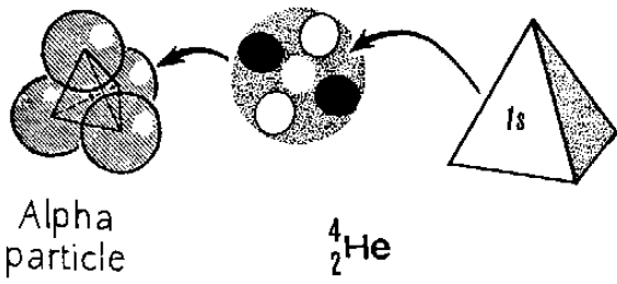
Fig.3. We represent the alpha-particle in several ways in this article. It is sometimes drawn as a ring (or "shell"), hollow in the centre, containing four nucleons. It is also useful to represent it as a three dimensional tetrahedron with a nucleon at each of its four corners. As the tetrahedron is hollow in its very centre, we can see why it makes sense to think of the alpha-particle as a shell rather than a spherical "core". The basic alpha-particle is also the 1s shell in the nuclear potential well of Fig.2, so we quite often simply draw a tetrahedron labelled 1s. It also corresponds to the "Magic Number" 1 because the 1s shell is filled by one alpha-particle.
